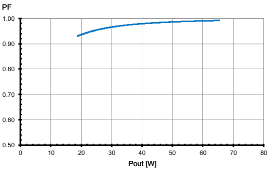
Power factor
