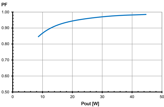
Power factor
